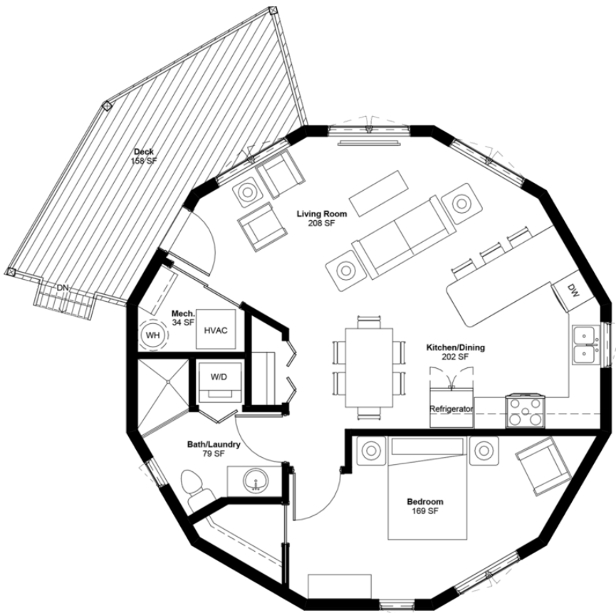
Shown on a crawlspace foundation with Deltec factory-installed high-performance engineered wood siding and optional covered roof over the deck.
